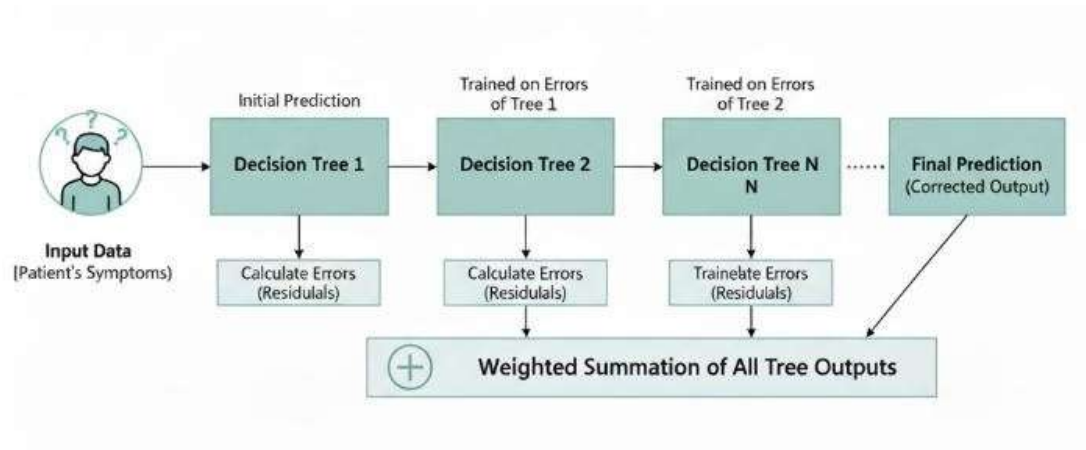
Figure 4: XGBoost Architecture
